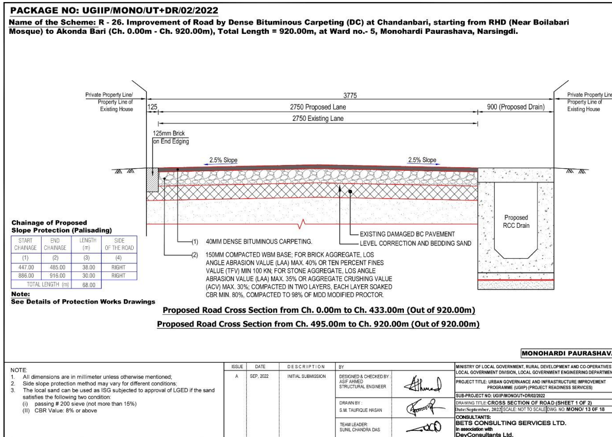
Figure-5: Cross-Section of Road
