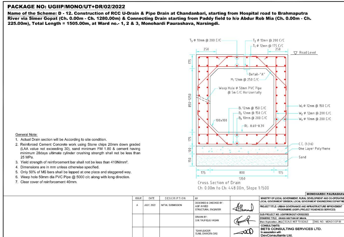
Figure-6: Cross-Section of Drain
